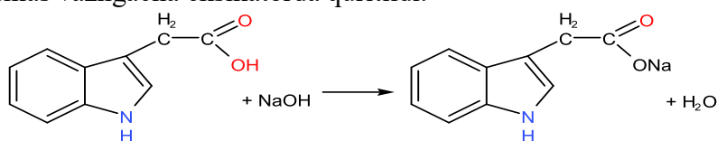
1-rasm. Geteroauksinning natriyli tuzini olish reaksiyasi
