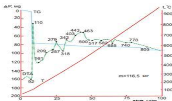
4-rasm. [\text{Mn}(\text{IAA})_2(\text{NIA})_2(\text{H}_2\text{O})_2] kompleks birikmasining derivatogrammasi
