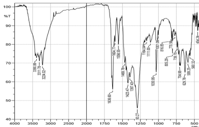
3-rasm. [\text{Mn}(\text{IAA})_2(\text{NIA})_2(\text{H}_2\text{O})_2] kompleks birikmasining IQ-spektri
