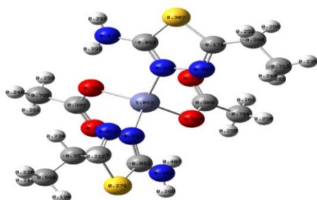
9-rasm. Bis(2-Amino-5-etil-1,3,4-tiadiazol)-diatsetato-rux(II) ( [\text{Zn}(\text{C}_4\text{H}_7\text{N}_3\text{S}_2)_2(\text{CH}_3\text{COO})_2] ) molekulasida elektron zaryadlarning taqsimlanishi
