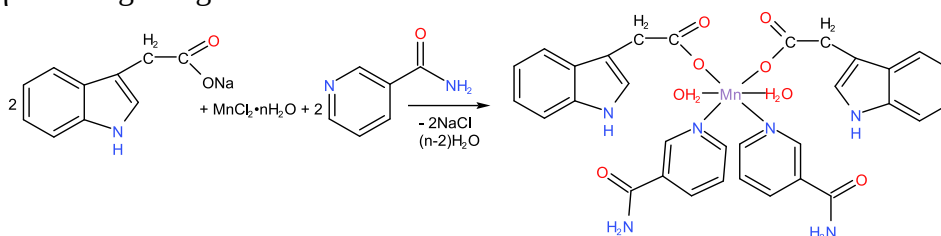
2-rasm. Geteroauksinning [\text{Mn}(\text{IAA})_2(\text{NIA})_2(\text{H}_2\text{O})_2] tarkibli kompleks birikmasining sintez reaksiyasi
