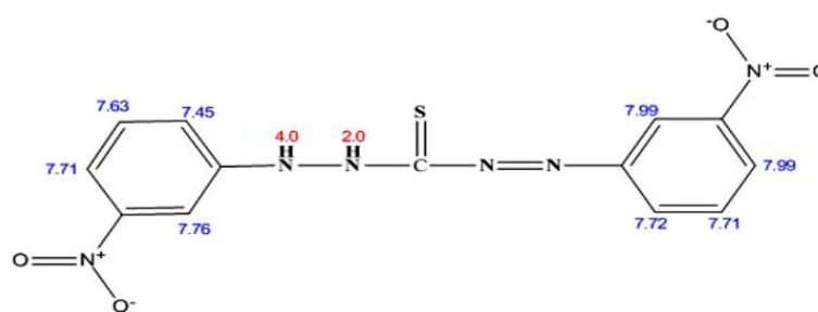
1,5-bis(3-nitrophenyl)thiocarbazono
