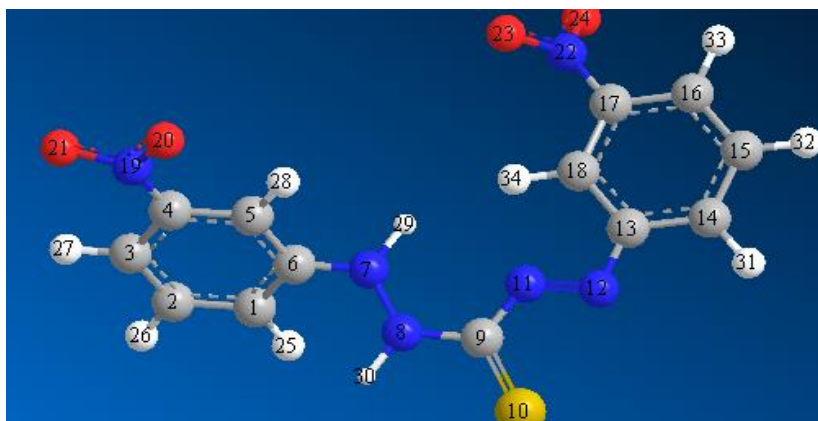
ChemNMR ^1\text{H} Estimation
