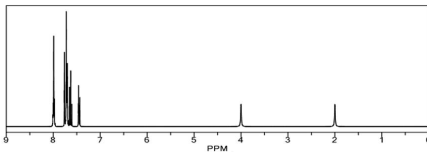
1,5-bis(3-nitrophenyl)thiocarbazono
